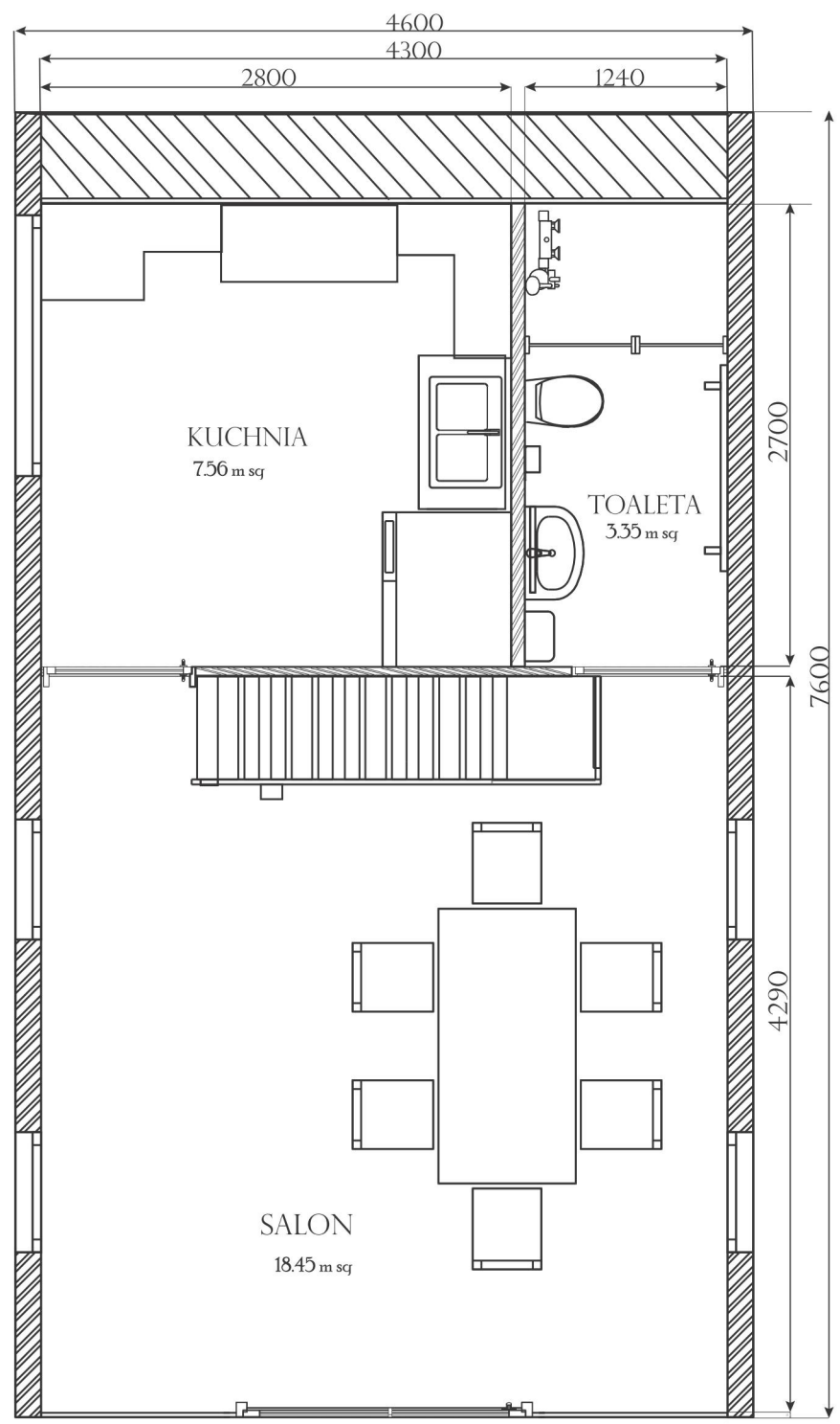
PLAN PARTERU
